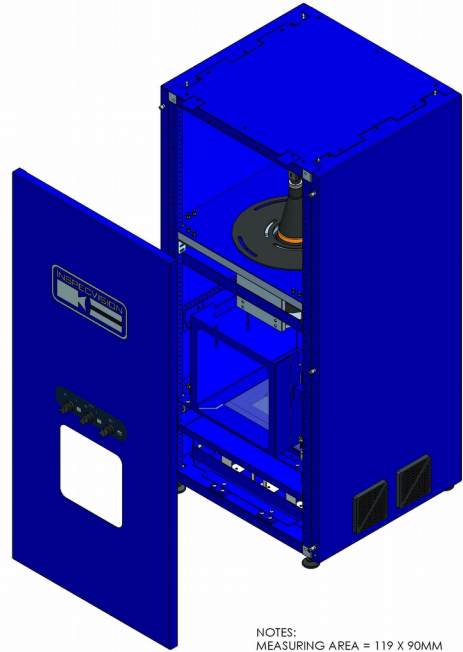
ISOMETRIC VIEW
